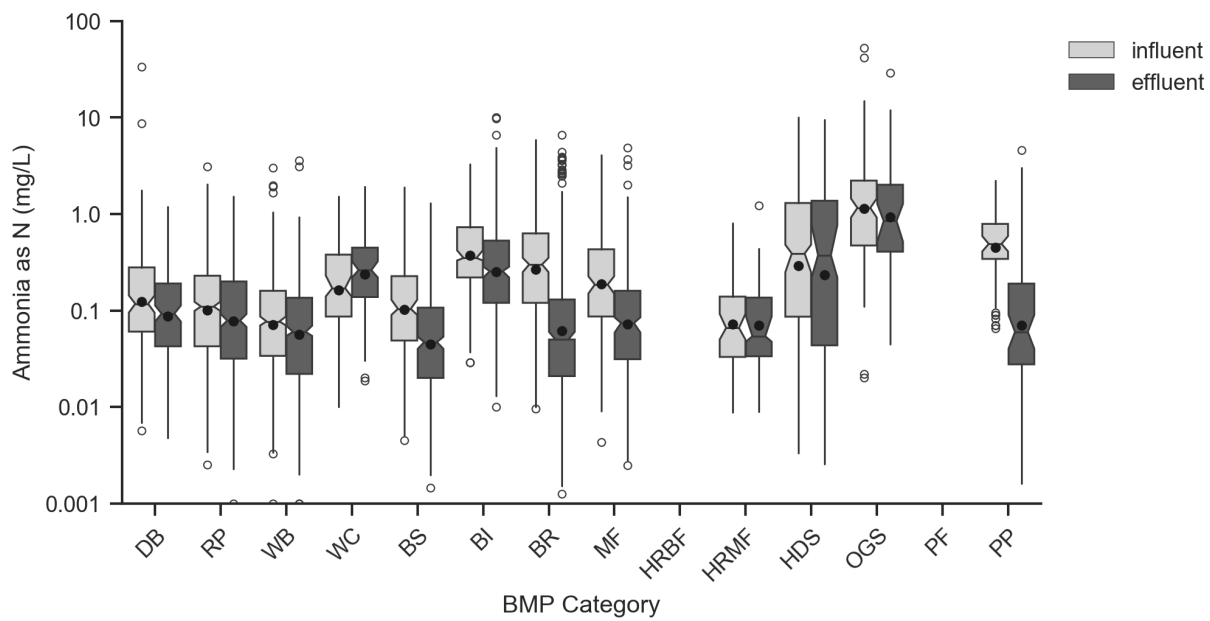
Figure 4-9. Box Plots of Influent/Effluent Ammonia as N (mg/L).
