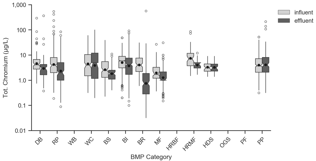
Figure 5-5. Box Plots of Influent/Effluent Total Chromium (µg/L).
