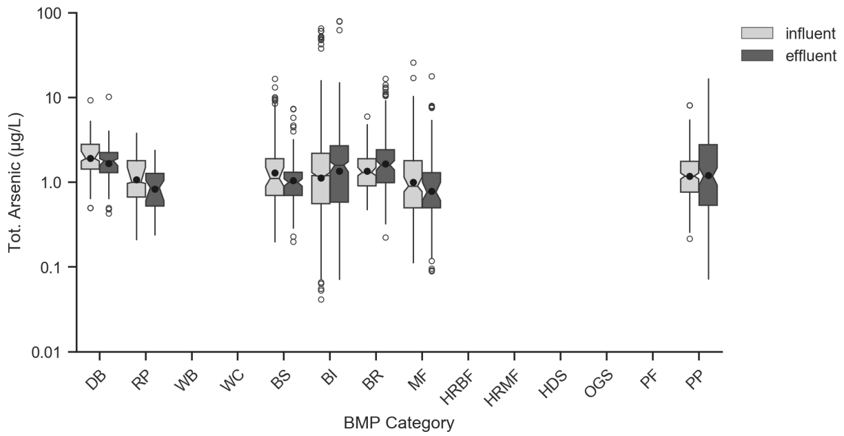
Figure 5-1. Box Plots of Influent/Effluent Total Arsenic (µg/L).
