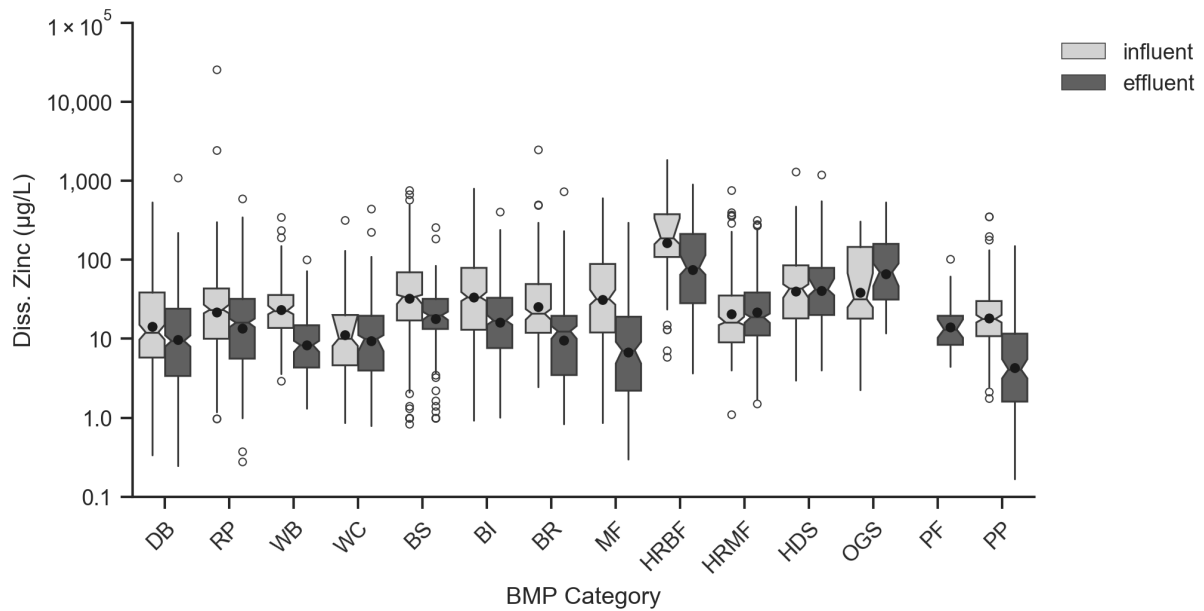
Figure 5-16. Box Plots of Influent/Effluent Dissolved Zinc (µg/L).
