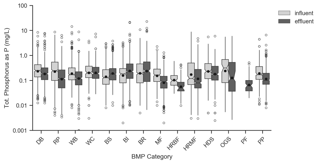
Figure 4-3. Box Plots of Influent/Effluent Total Phosphorus as P (mg/L).
