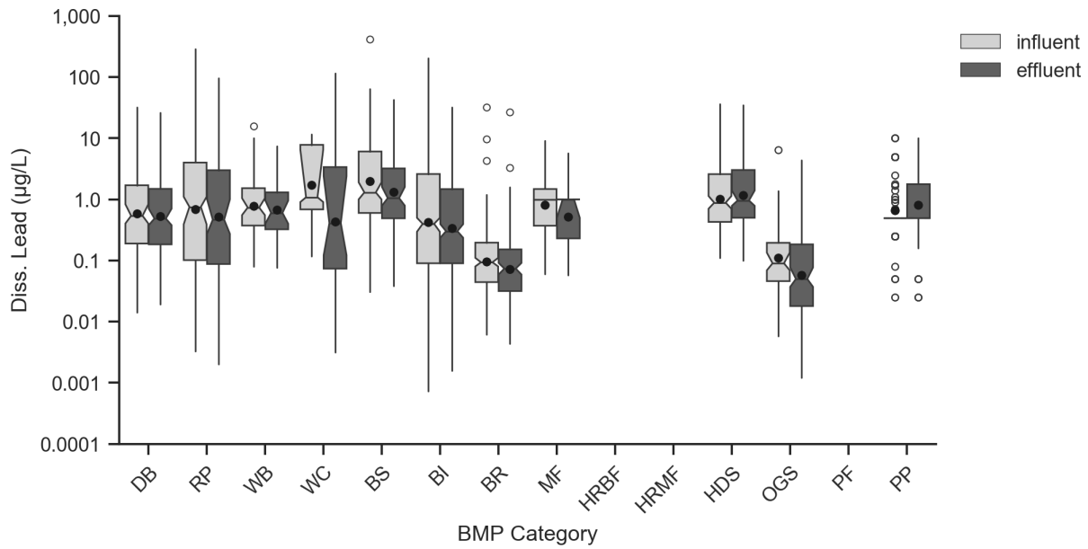
Figure 5-12. Box Plots of Influent/Effluent Dissolved Lead (µg/L).
