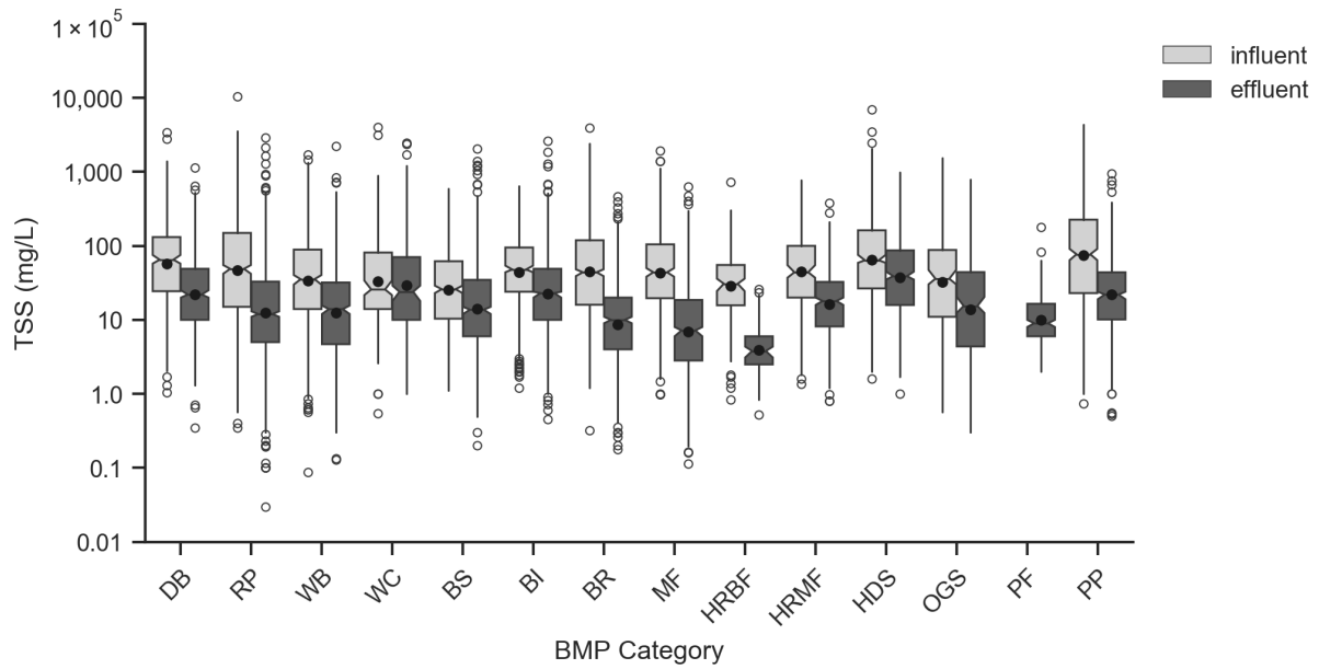
Figure 2-2. Box Plots of Influent/Effluent TSS (mg/L).
