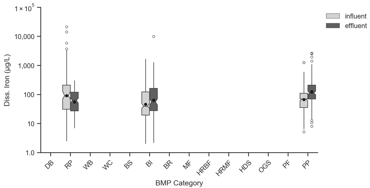
Figure 5-10. Box Plots of Influent/Effluent Dissolved Iron (µg/L).
