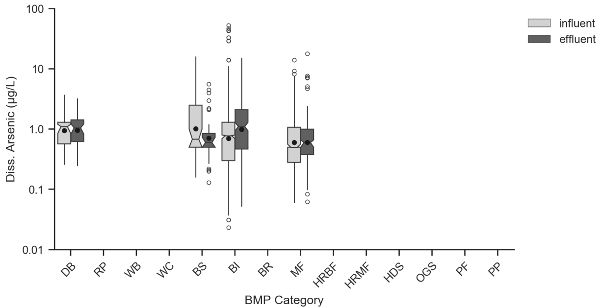
Figure 5-2. Box Plots of Influent/Effluent Dissolved Arsenic (µg/L).
