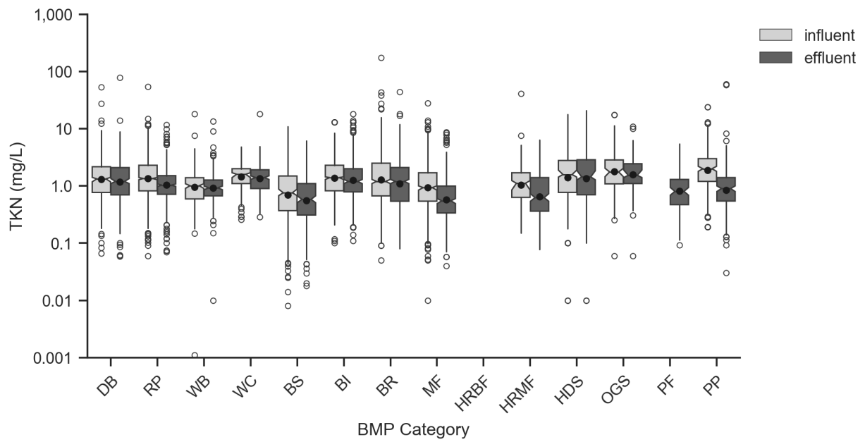
Figure 4-7. Box Plots of Influent/Effluent TKN (mg/L).
