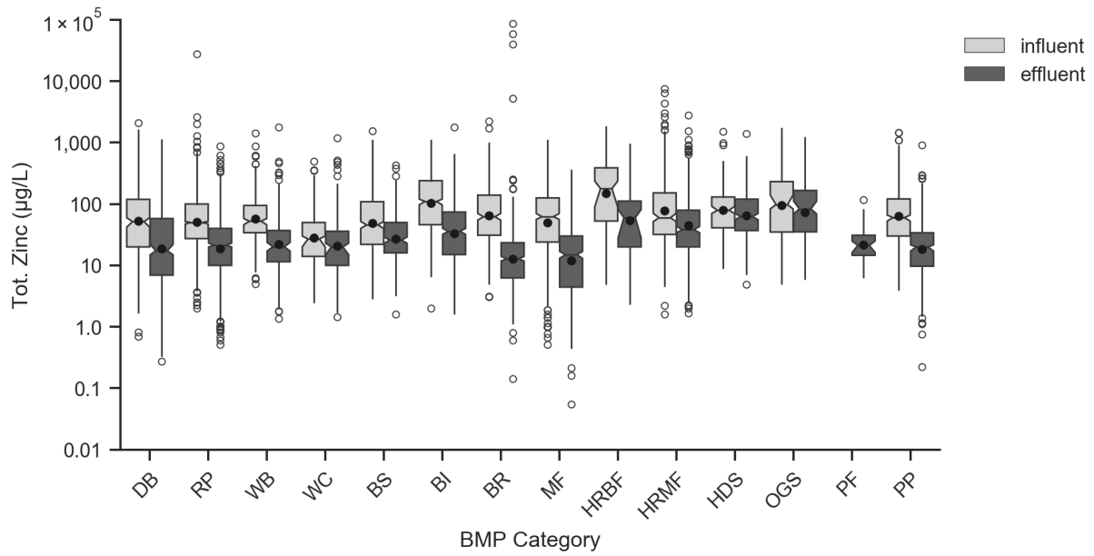
Figure 5-15. Box Plots of Influent/Effluent Total Zinc (µg/L).
