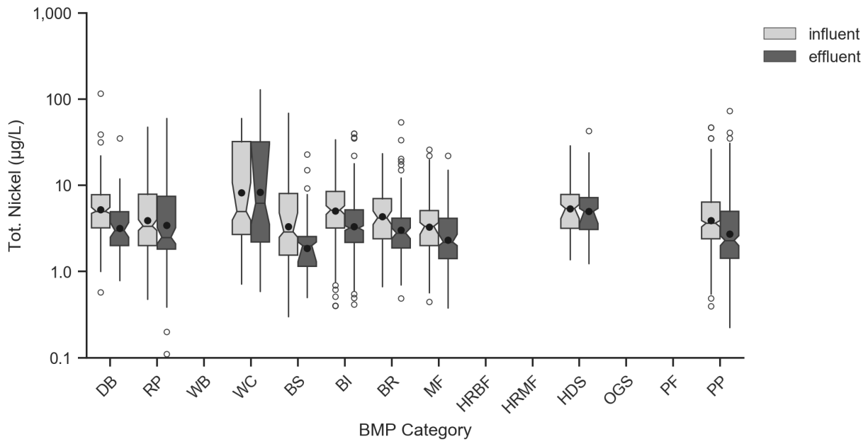
Figure 5-13. Box Plots of Influent/Effluent Total Nickel (µg/L).
