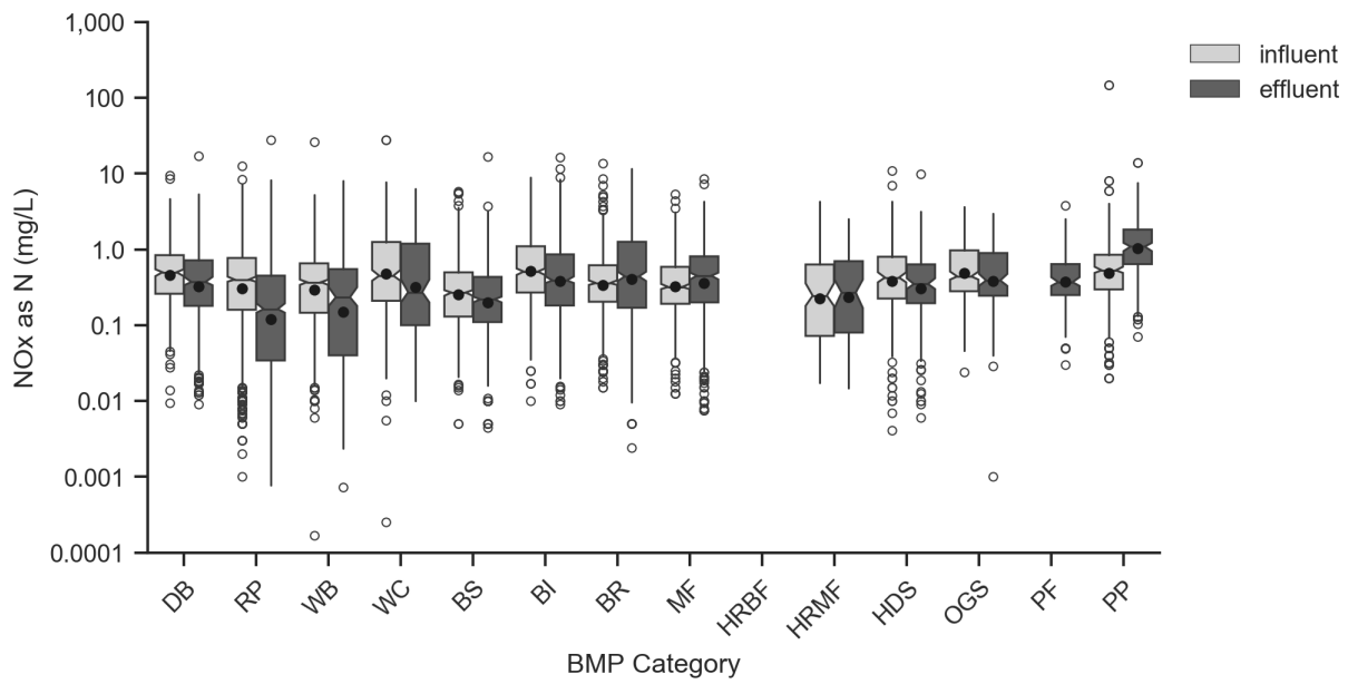
Figure 4-8. Box Plots of Influent/Effluent NOx as N (mg/L).
