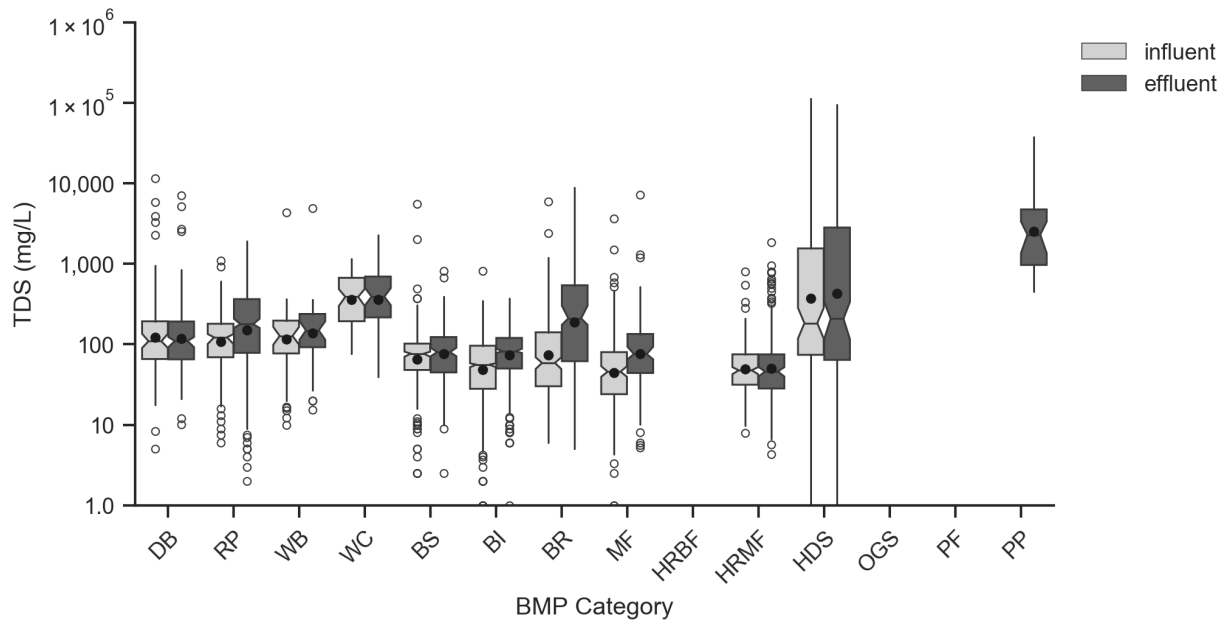
Figure 2-3. Box Plots of Influent/Effluent TDS (mg/L).
