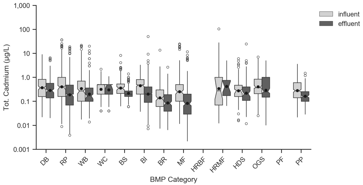
Figure 5-3. Box Plots of Influent/Effluent Total Cadmium (µg/L).
