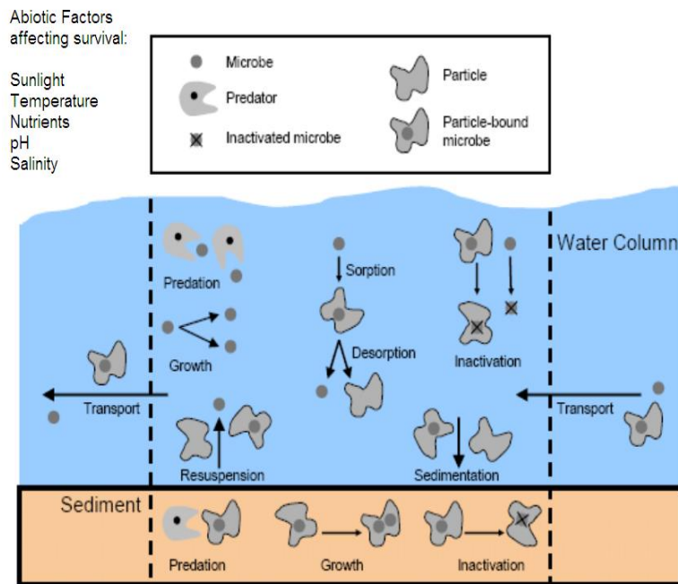
Figure 3-1. Potential Factors that Impact Fate of Microorganisms in Waterbodies and Associated Sediment.
