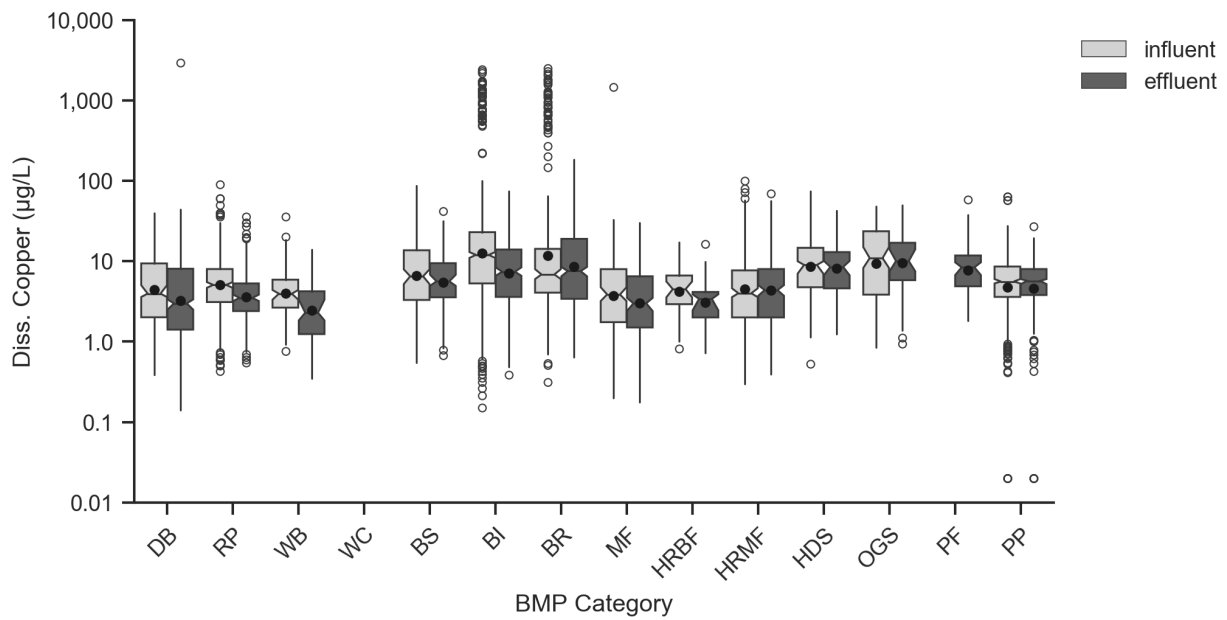
Figure 5-8. Box Plots of Influent/Effluent Dissolved Copper (µg/L).
