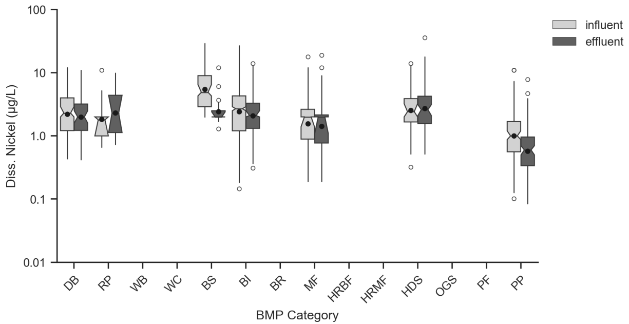
Figure 5-14. Box Plots of Influent/Effluent Dissolved Nickel (µg/L).
