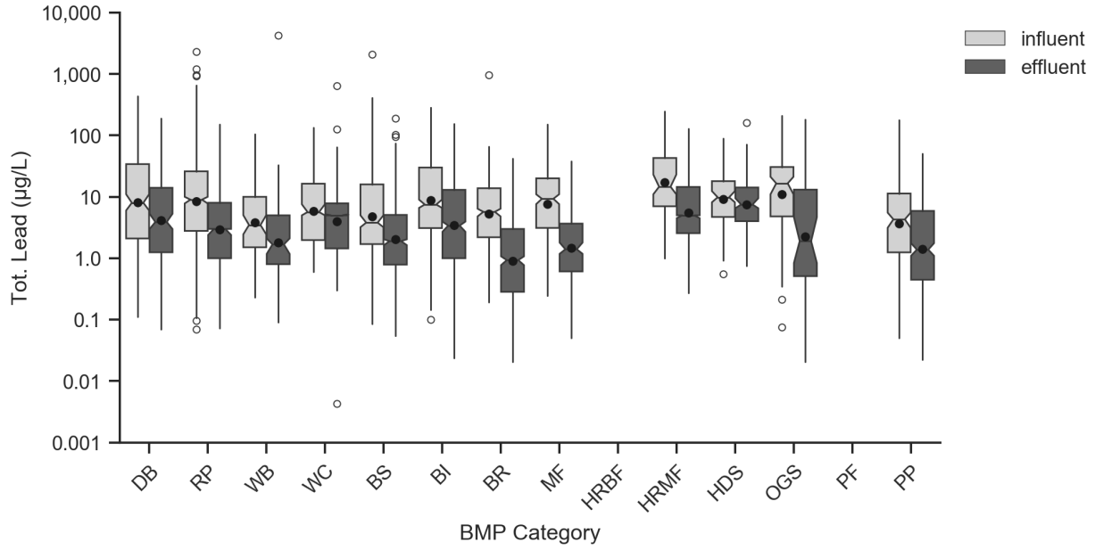
Figure 5-11. Box Plots of Influent/Effluent Total Lead (µg/L).
