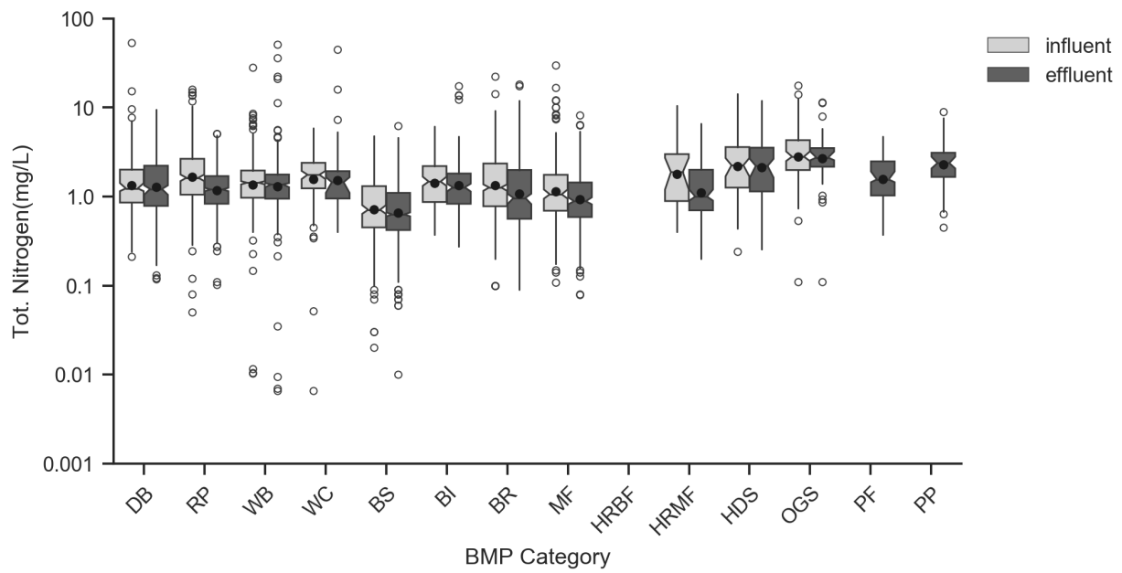
Figure 4-6. Box Plots of Influent/Effluent Total Nitrogen (mg/L).
