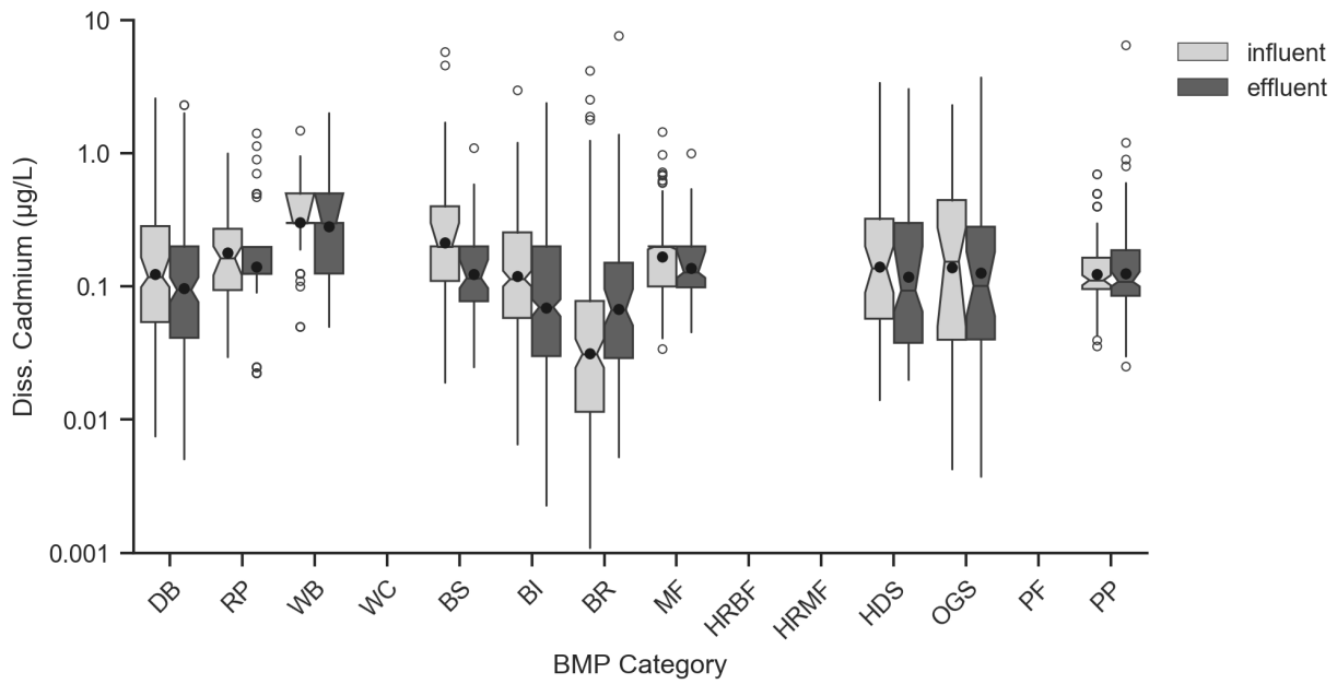
Figure 5-4. Box Plots of Influent/Effluent Dissolved Cadmium (µg/L).
