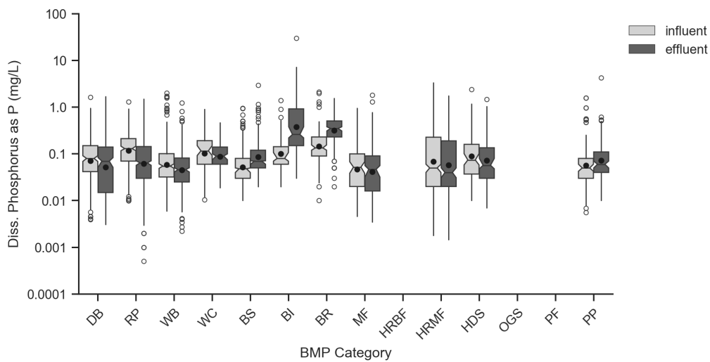
Figure 4-5. Box Plots of Influent/Effluent Dissolved Phosphorus as P (mg/L).
