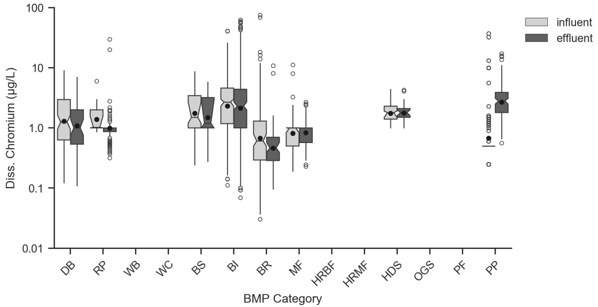
Figure 5-6. Box Plots of Influent/Effluent Dissolved Chromium (µg/L).
