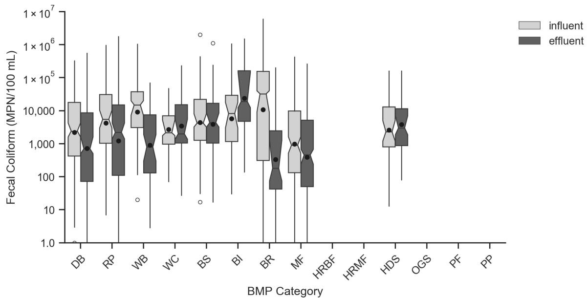
Figure 3-4. Box Plots of Influent/Effluent Fecal Coliform (cfu/100 mL).
