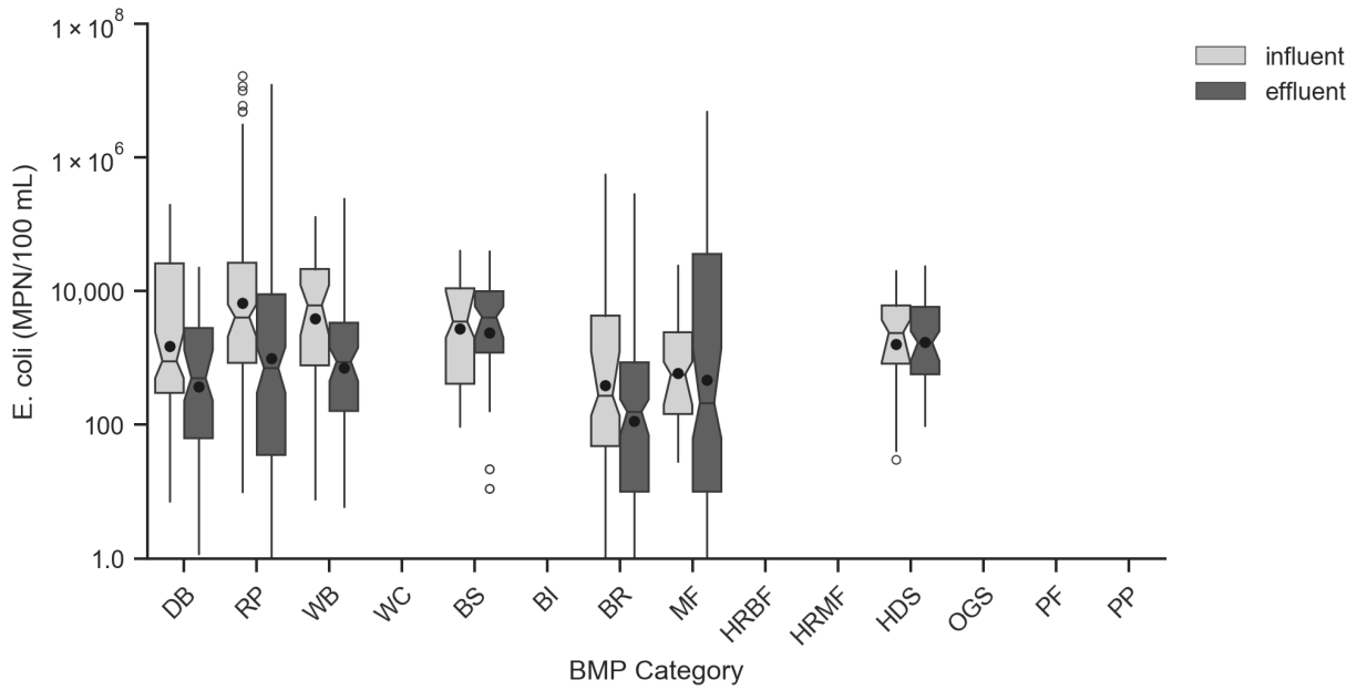
Figure 3-2. Box Plots of Influent/Effluent E. coli (MPN/100 mL).
