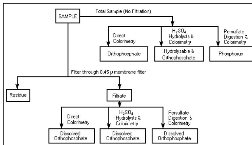
Figure 4-1. Analytical Procedure for the Differentiation of Phosphorus Forms.
