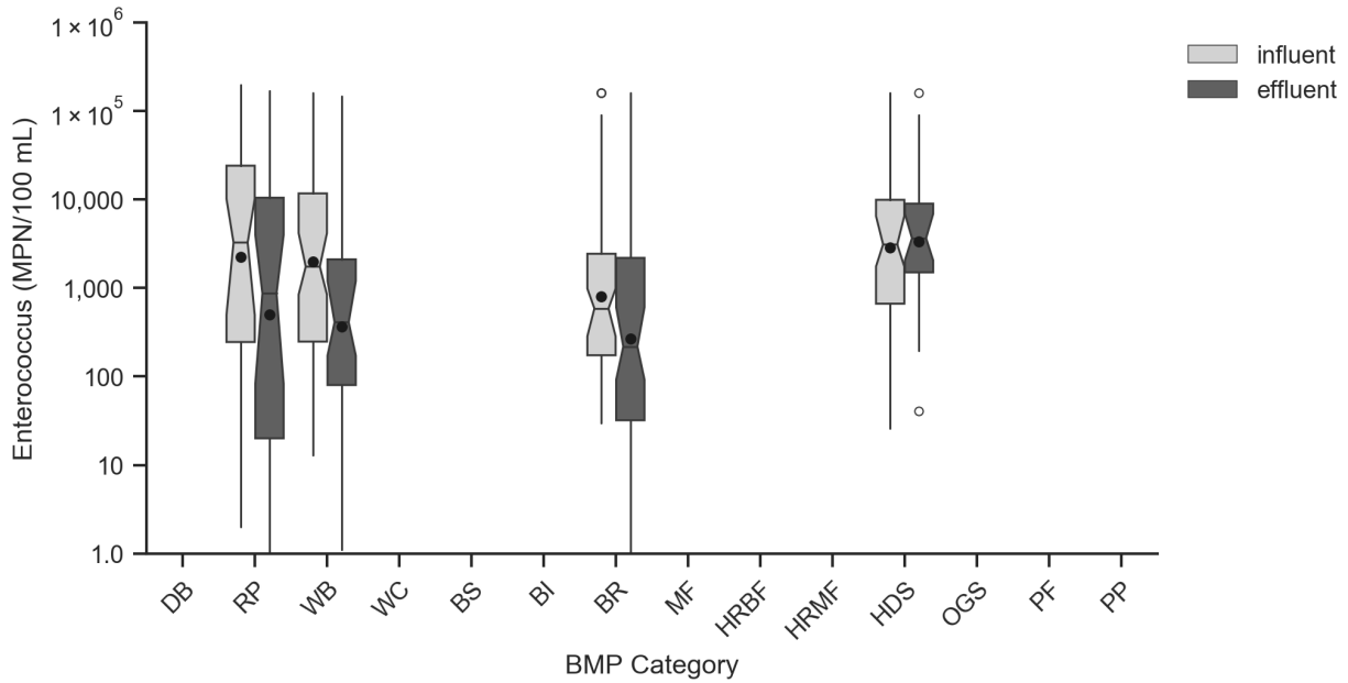
Figure 3-3. Box Plots of Influent/Effluent Enterococcus (MPN/100 mL).
