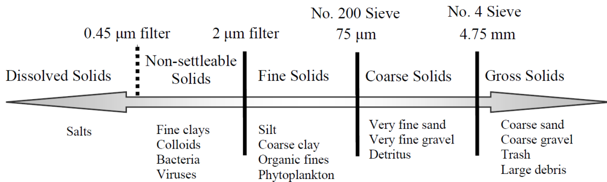
Figure 2-1. Solids Classification Scheme.
