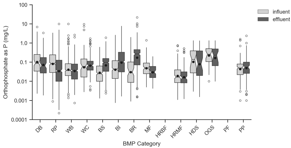
Figure 4-4. Box Plots of Influent/Effluent Orthophosphate as P (mg/L).
